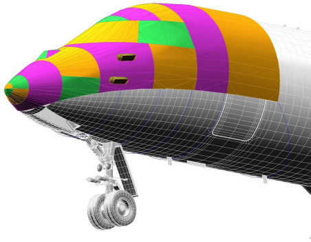
Bombardier Global Express Cockpit/Nose Cover, 3D model
